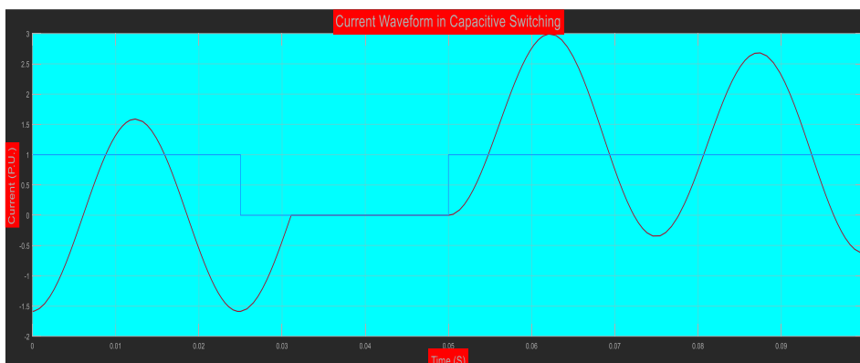
Fig. 4.5 Current Waveform in Capacitive Switching in One Phase
