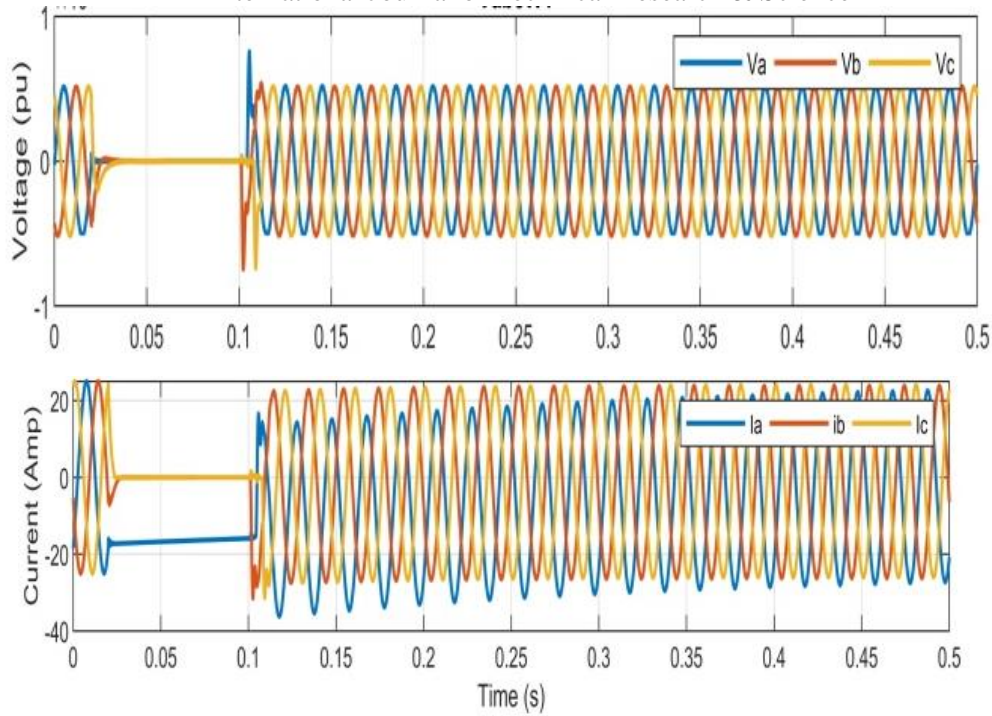
Fig. 4.3 Voltage and Current Waveform Respectively during the Three Phase fault d.) Capacitive Switching Events
