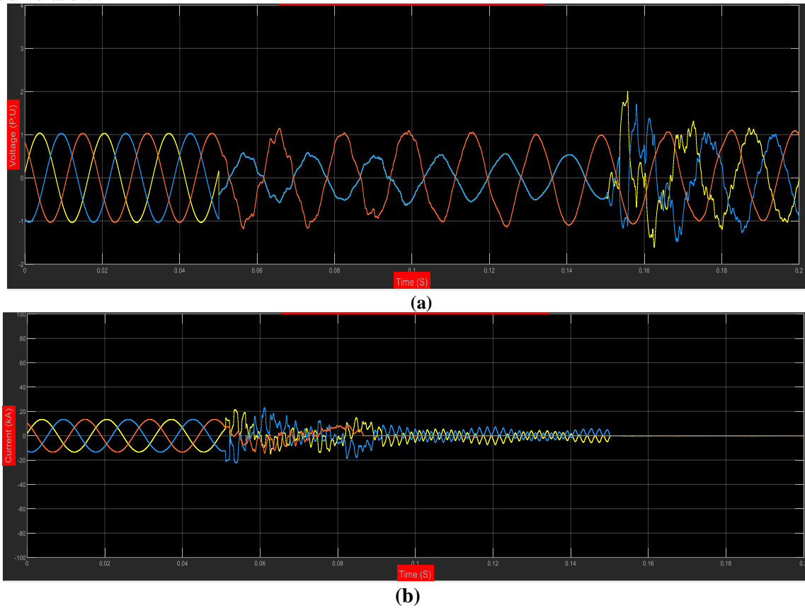
Fig. 4.1 (a), (b) Voltage and Current Waveforms Respectively during Power Electronic Loading
