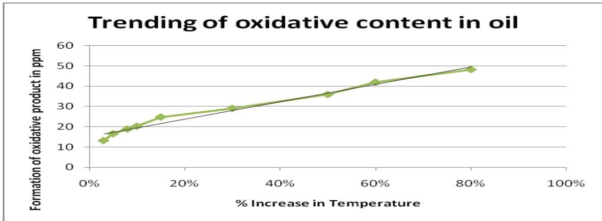
Fig. 4.7 Formation of Oxidative Content with Traditional Method
