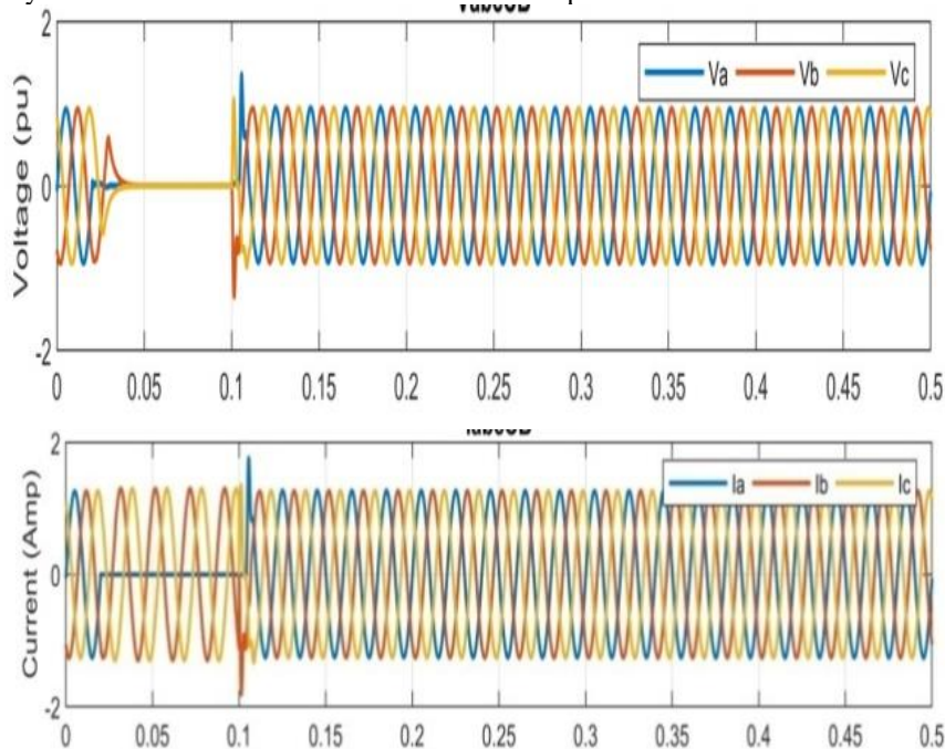
Fig. 4.2 Voltage and Current Waveform Respectively During the Single-Phase Fault
