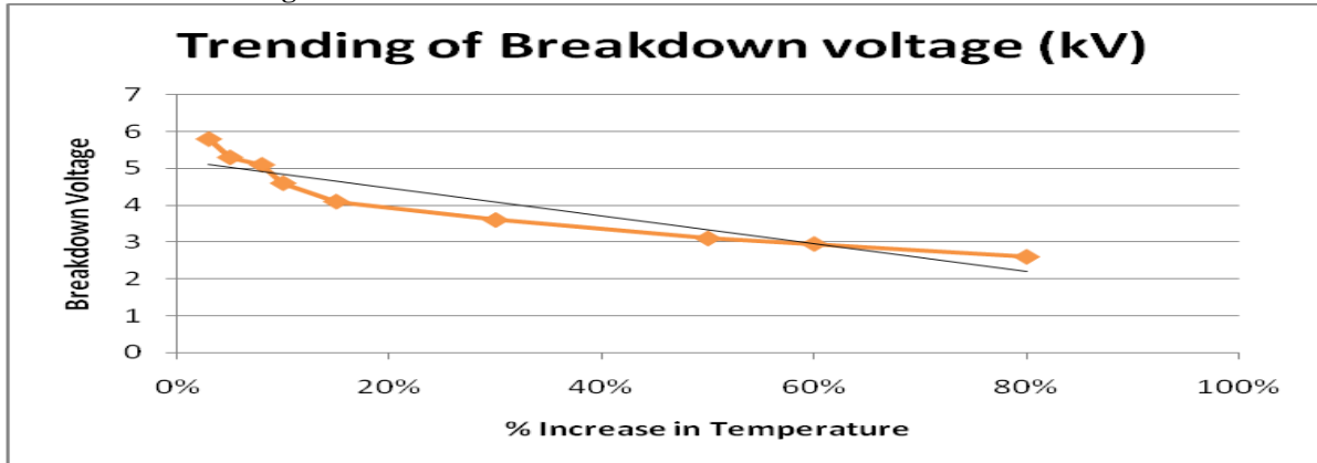
Fig. 4.8 Breakdown Voltage of Oil with Traditional Method
