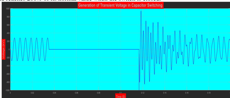
Fig. 4.4 Generation of Transient Voltage in Capacitor Switching in one Phase
