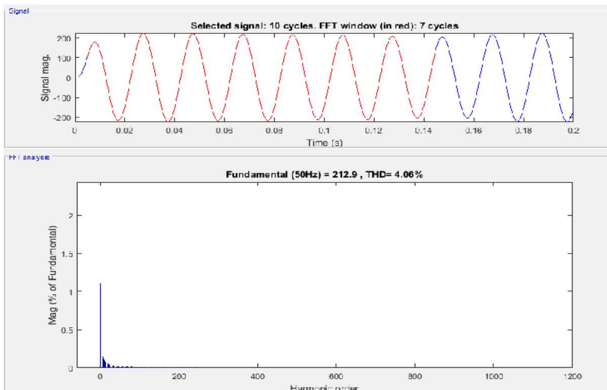
(b) Harmonic spectrum of output load voltage
