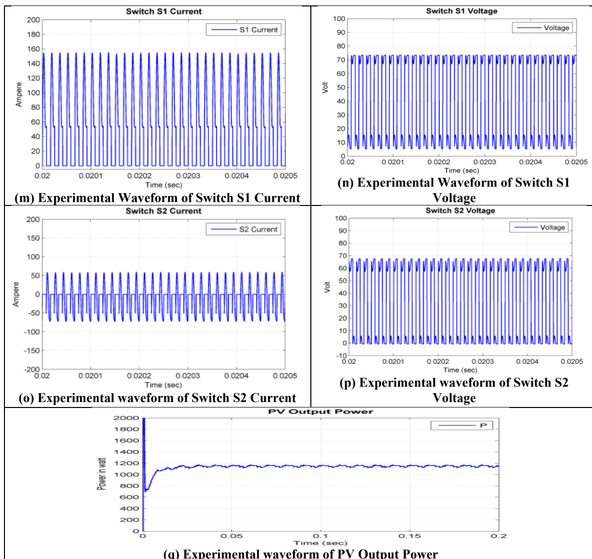
Fig. a. Experimental Waveforms during Constant Resistive Load of 1 kW at 600 Irradiance and 25° C Temperature
