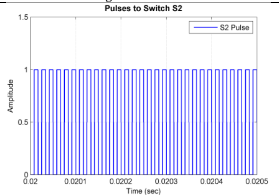
(l). Experimental waveform of Pulses to Switch S2.
