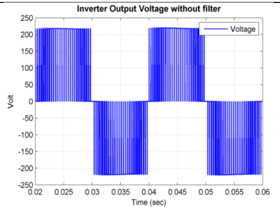
(j) Experimental Waveform of Inverter Output Voltage Without Filter
