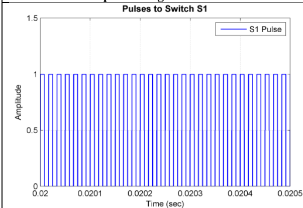
(k). Experimental waveform of Pulses to Switch S1.
