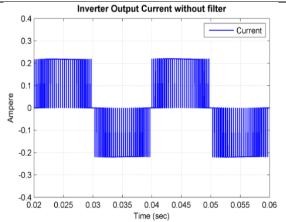
(h) Experimental waveform of Inverter Output Current without filter
