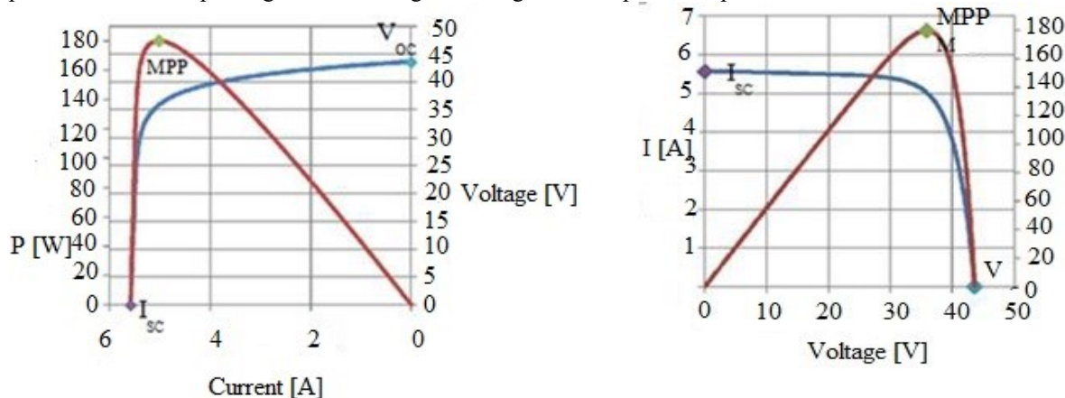
Fig. 2.3 PV Panel Characteristic Curves
