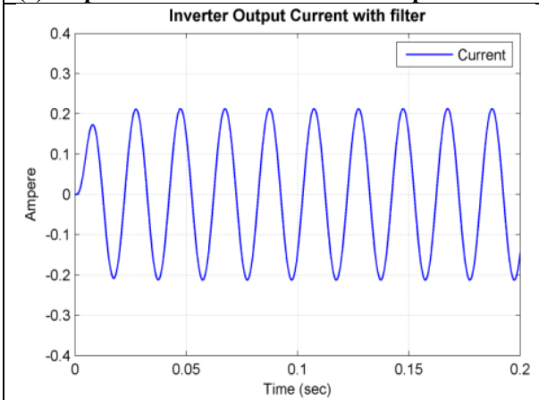
(g) Experimental waveform of Inverter Output Current with filter
