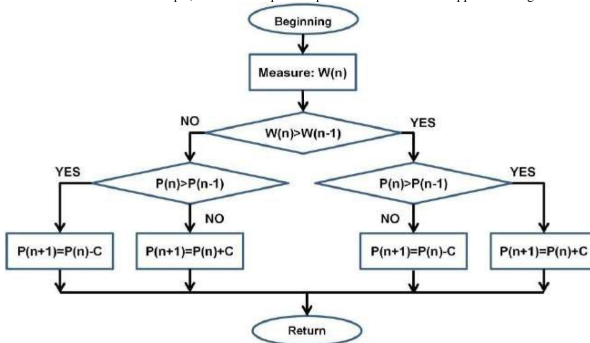
Fig. 2.4 Flow Chart P & O Method MPPT
