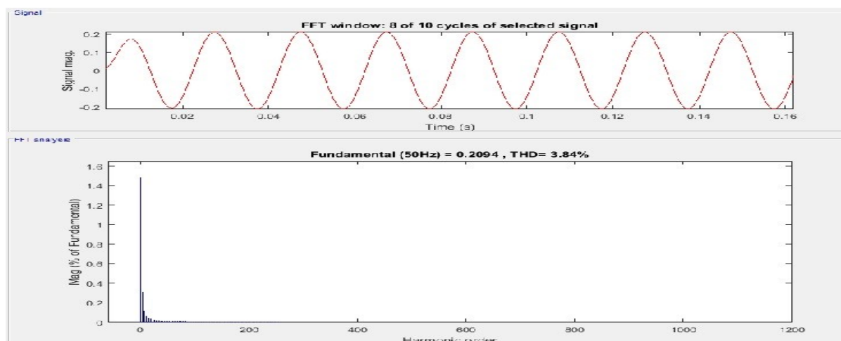
(a) Harmonic Spectrum of Output Load Current
