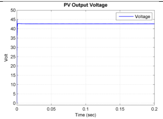
(f). Experimental waveform of PV Output Voltage.
