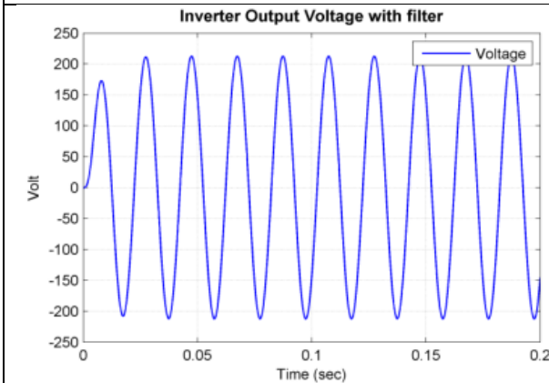
(i) Experimental Waveform of Inverter Output Voltage with Filter
