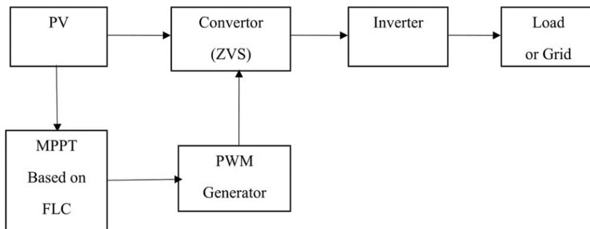
Fig. 2.1 Block Diagram of PV Standalone System with ZVS
