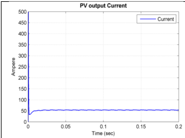
(e). Experimental waveform of PV Output Current.
